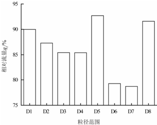
图 4 粒径与灌水器相对流量关系 Fig.4 Impact of particle size distribution on relative flow
