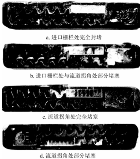
图 3 迷宫流道堵塞情形 Fig.3 Illustration of emitter clogging in labyrinth-channels
